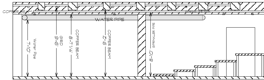
FRONT ELEVATION
