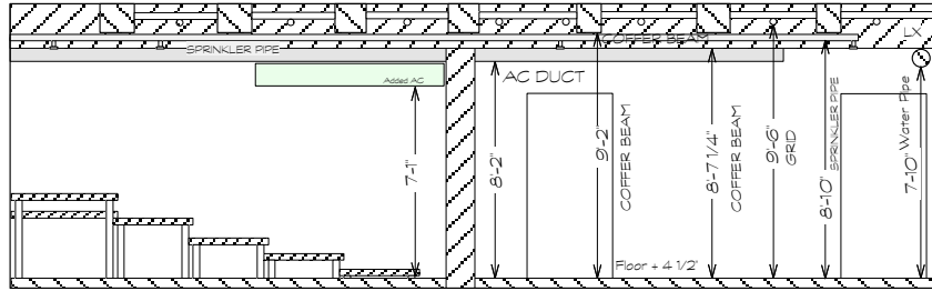
SL SECTION
