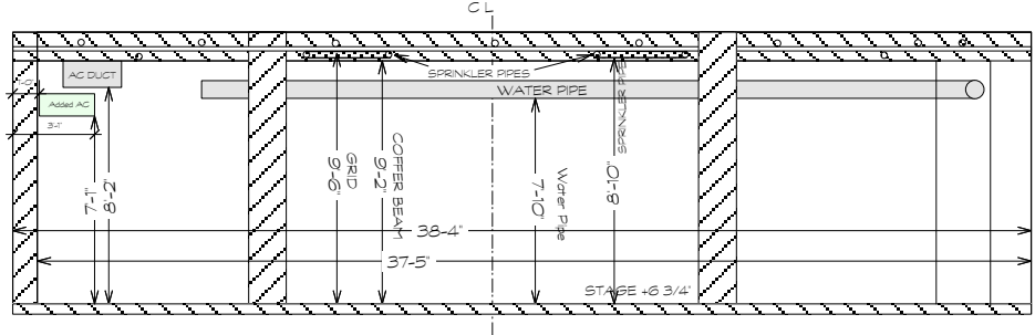
FRONT ELEVATION
